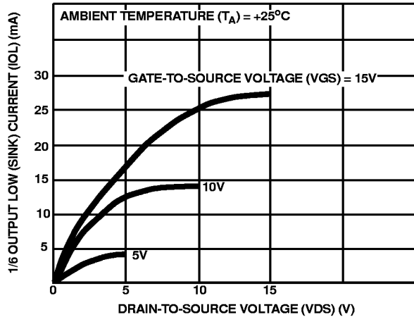
FIGURE 1. TYPICAL OUTPUT LOW (SINK) CURRENT CHARACTERISTICS
