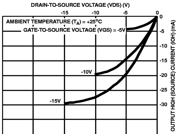
FIGURE 3. TYPICAL OUTPUT HIGH (SOURCE) CURRENT CHARACTERISTICS
