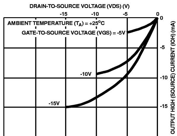
FIGURE 4. MINIMUM OUTPUT HIGH (SOURCE) CURRENT CHARACTERISTICS
