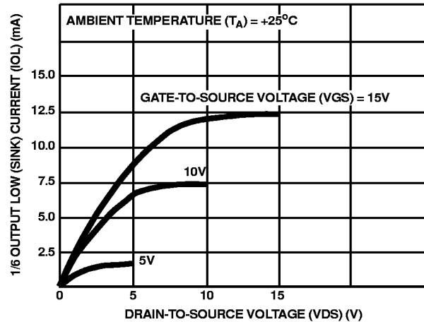
FIGURE 2. MINIMUM OUTPUT LOW (SINK) CURRENT CHARACTERISTICS
