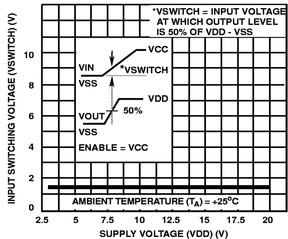
FIGURE 6. TYPICAL INPUT SWITCHING AS A FUNCTION OF HIGH LEVEL SUPPLY VOLTAGE (SELECT AT VSS-TTL MODE)
