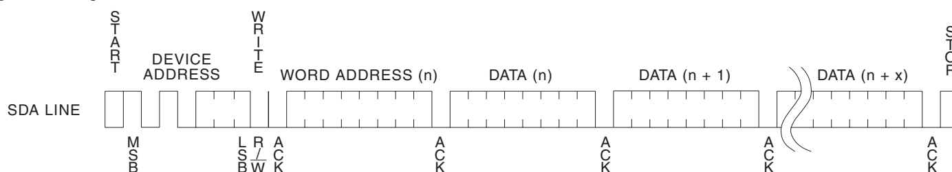
Figure 9. Page Write
