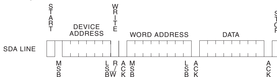
Figure 8. Byte Write
