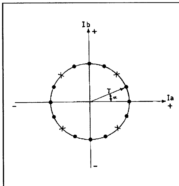
Figure 7. Microstepping
