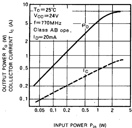
OUTPUT POWER, COLLECTOR CURRENT VS. INPUT POWER
