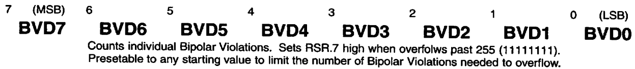
Figure 24. Bipolar Violation Count Register (BVCR)
