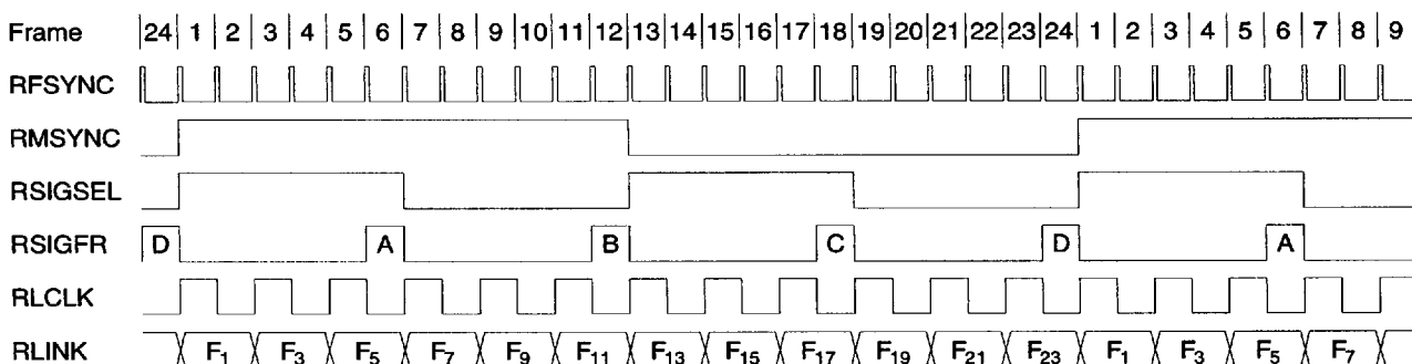
Figure 16. 193E Multiframe Receive Timing
