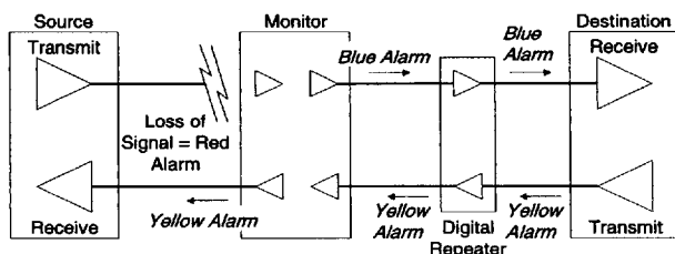
Figure A10. Alarm Operation on a T1 Link.
