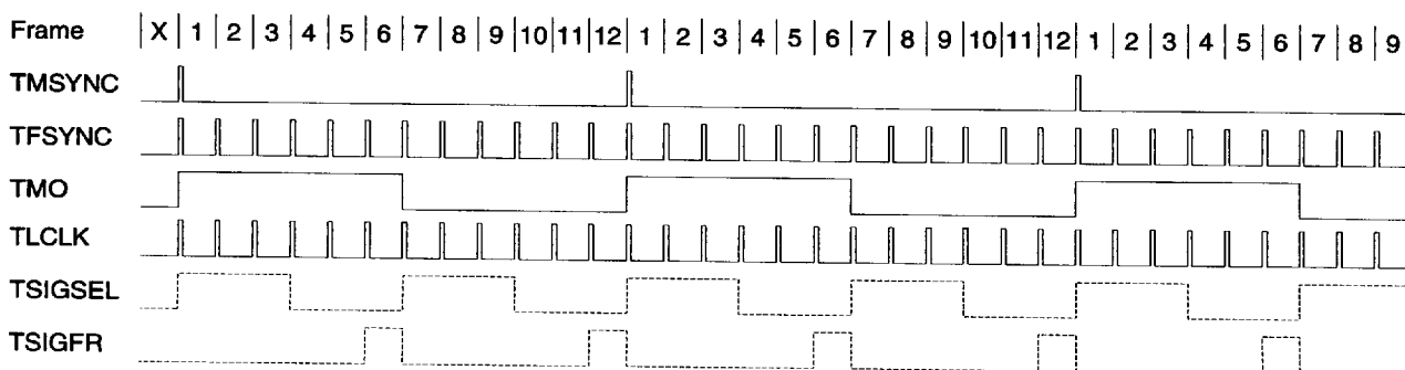
Figure 9. T1DM Multiframe Transmit Timing
