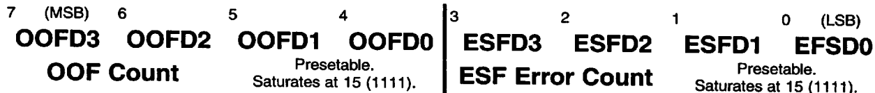
Figure 23. Error Count Register (ECR)
