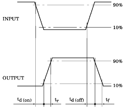
WAVEFORMS
