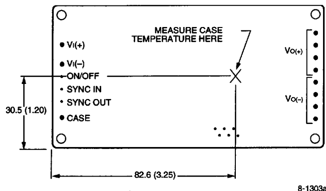
Figure 4. Case Temperature Measurement Location
