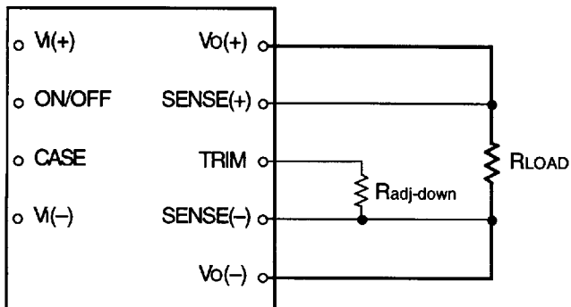
Figure 7. Circuit Configuration to Decrease Output Voltage
