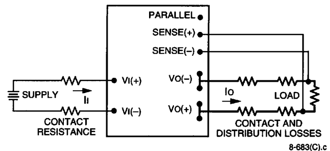
Figure 5. Effective Circuit Configuration for Single-Module Remote-Sense Operation
