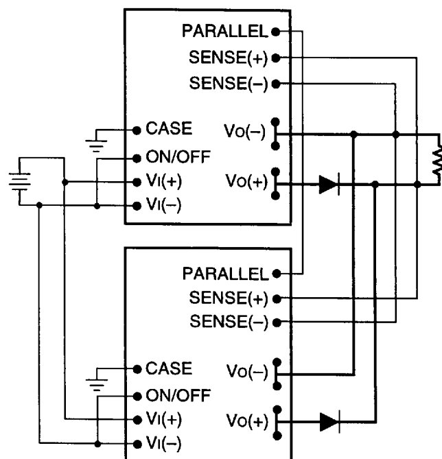
Figure 6. Wiring Configuration for Redundant Parallel Operation
