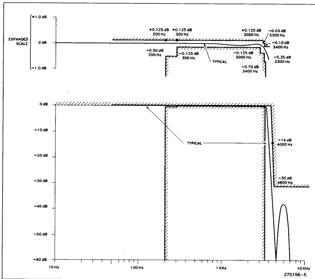
Figure 5. Receive Channel
