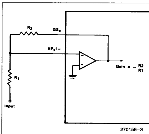
Figure 3. Transmit Filter Gain Adjustment
