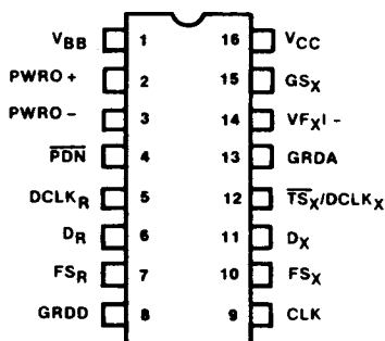
Figure 1. Pin Configuration
