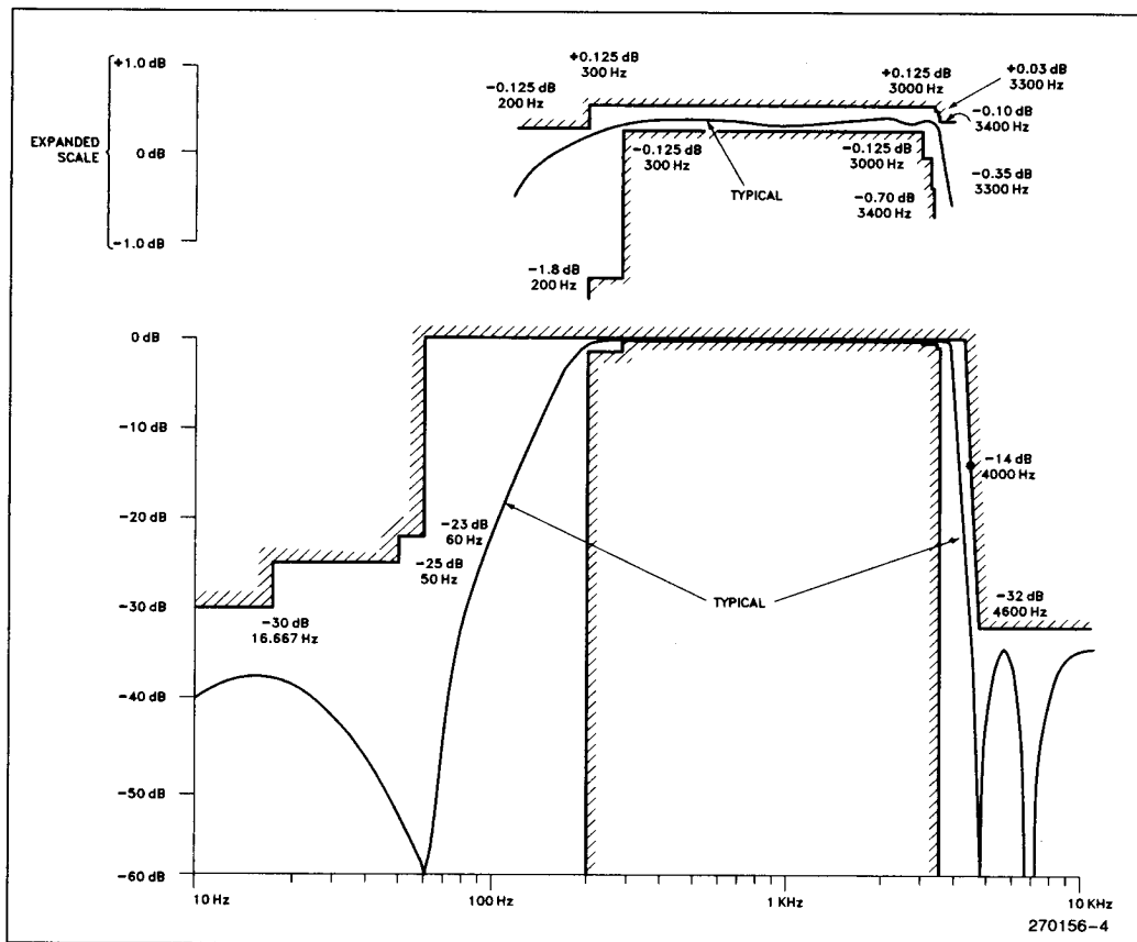
Figure 4. Transmit Channel
