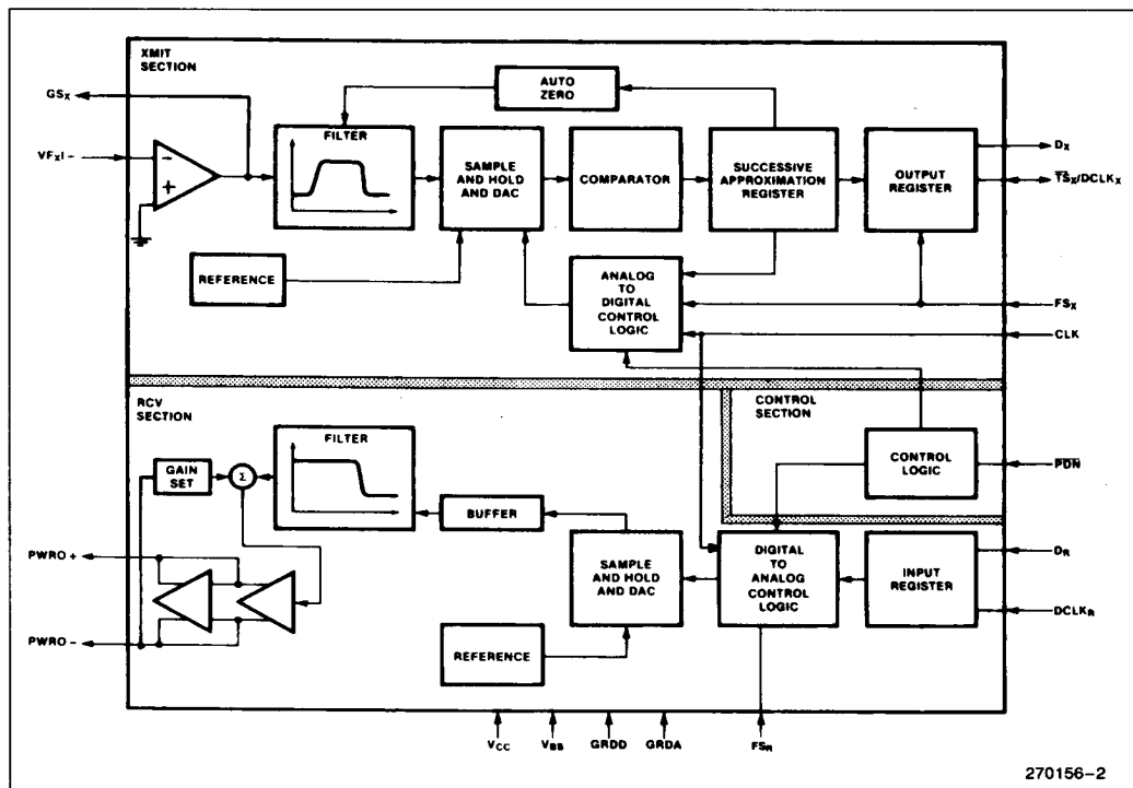
Figure 2. Block Diagram
