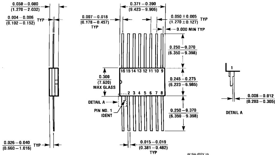
16-Lead Ceramic Flat Package (W) Order Number 54151AFMQB or DM54151AW NS Package Number W16A
