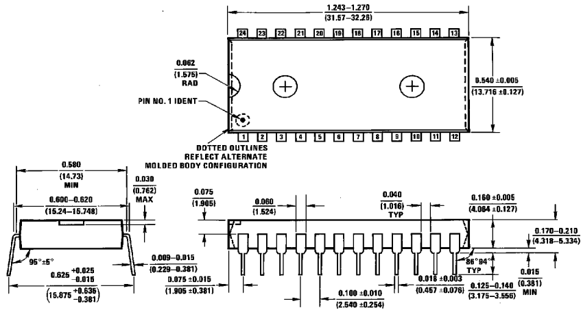
24-Lead Molded Dual-In-Line Package (N) Order Number DM74150N NS Package Number N24A
