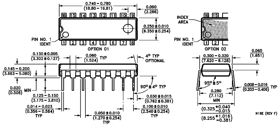
16-Lead Molded Dual-In-Line Package (N) Order Number DM74151AN NS Package Number N16E
