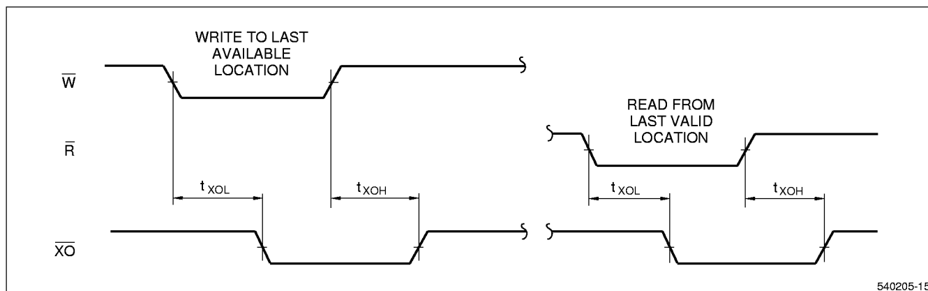
Figure 19. Expansion-Out Timing
