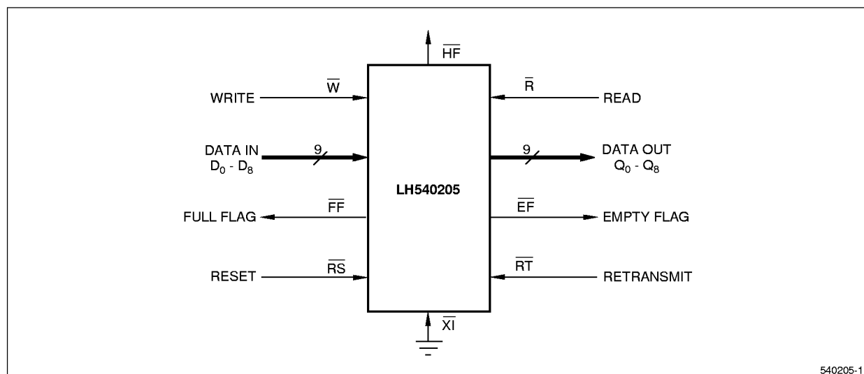
Figure 3. Standalone FIFO (8192 × 9)
