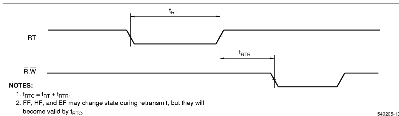
Figure 18. Retransmit Timing
