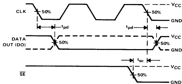
FIGURE 2. DATA OUTPUT TIMING
