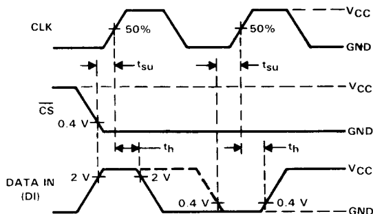
FIGURE 1. DATA INPUT TIMING
