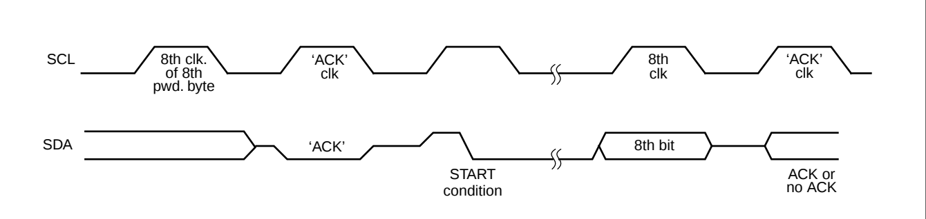
Figure 5. Acknowledge Polling
