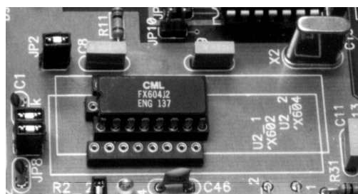
Figure 4 FX604 Configuration
