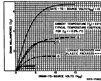
Fig. 4—Minimum output n-channel drain characteristics.
