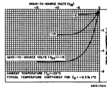
Fig. 5—Typical output p-channel drain characteristics.
