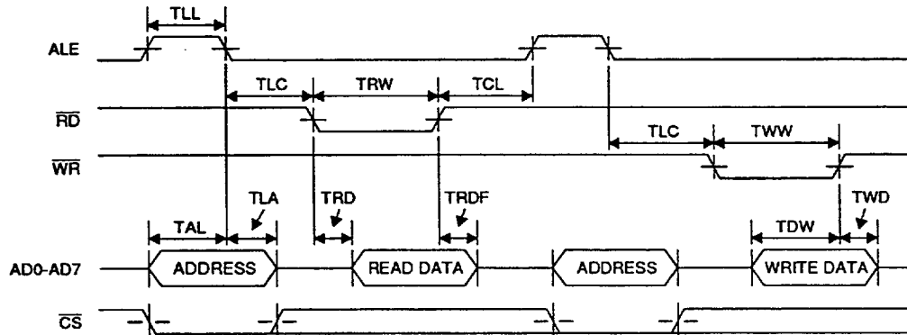
BUS TIMING DIAGRAM (PARALLEL VERSION)
