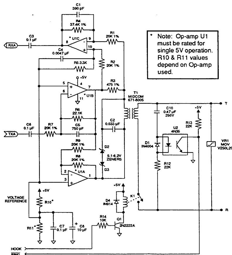
FIGURE 2: Single 5V Hybrid Version
