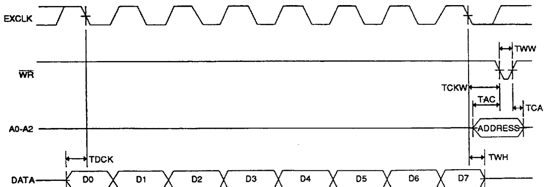
WRITE TIMING DIAGRAM (SERIAL VERSION)
