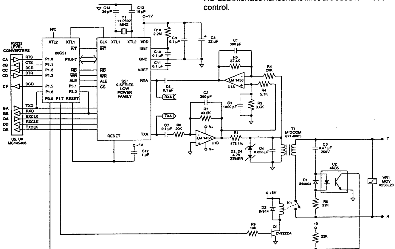
FIGURE 1: Basic Box Modem with Dual-Supply Hybrid
