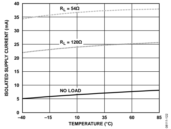
Figure 22. ADM2687E Isolated Supply Current vs. Temperature ( V_{CC} = 3.3\text{ V} , Data Rate = 500 kbps)
