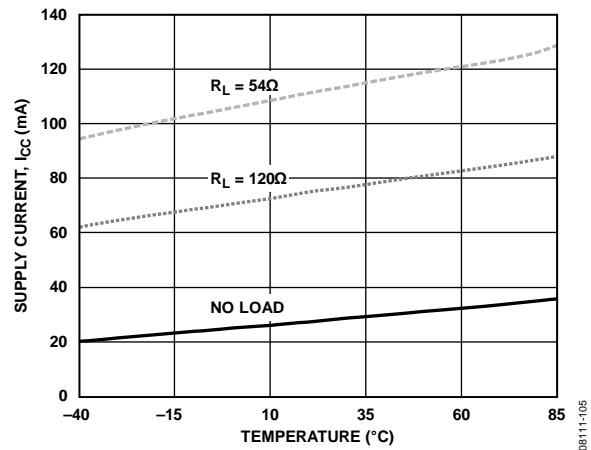
Figure 6. ADM2687E Supply Current ( I_{CC} ) vs. Temperature (Data Rate = 500 kbps, DE = 3.3 V, V_{CC} = 3.3 V)
