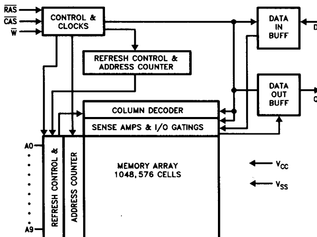
Figure 1. Block Diagram
