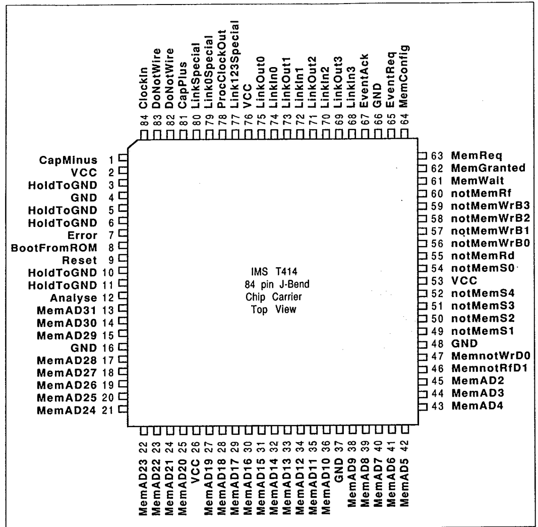
Figure 11.3: IMS T414 84 pin PLCC J-bend package pinout
