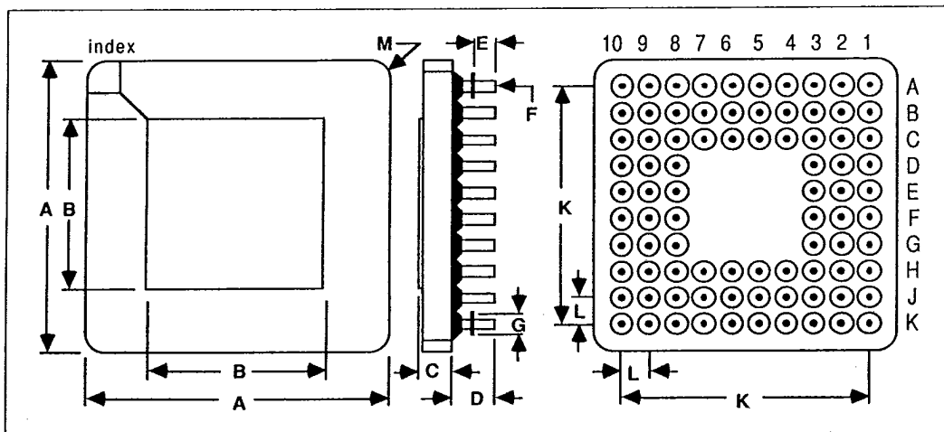
Figure 11.2: 84 pin grid array package dimensions
