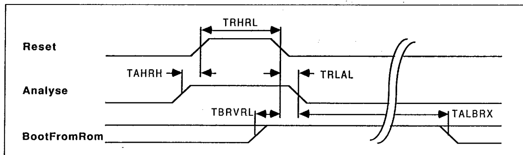
Figure 5.5: Transputer reset and analyse timing
