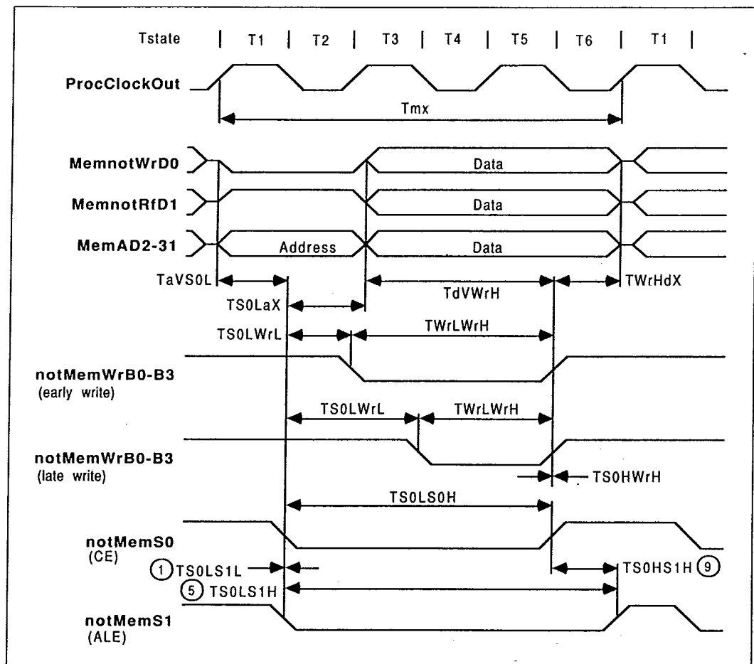
Figure 7.7: IMS T414 external write cycle
