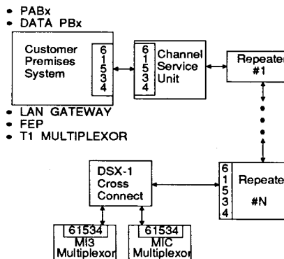
Figure A5. Application of CS61534
