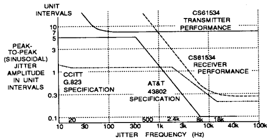
Figure 10. Typical Input Jitter Tolerance
