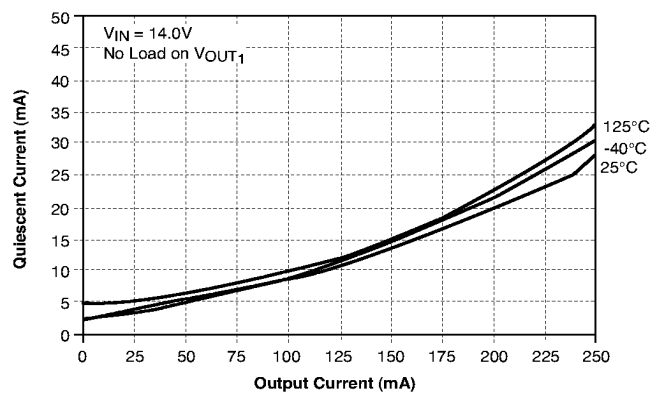
Quiescent Current vs Output Current for V_{OUT2}
