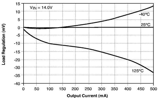
Load Regulation vs. Output Current for V_{OUT1}
