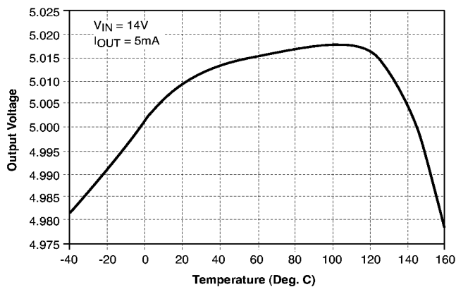
Output Voltage vs. Temperature for V_{OUT2}
