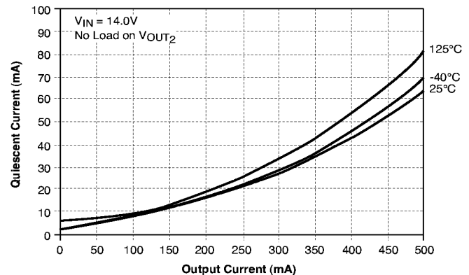
Quiescent Current vs. Output Current for V_{OUT1}
