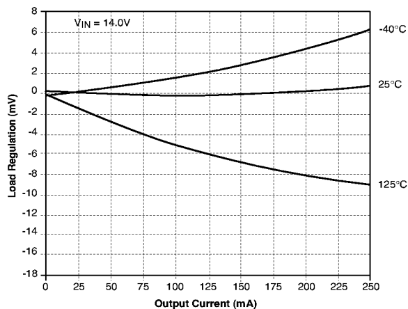
Load Regulation vs Output Current for V_{OUT2}
