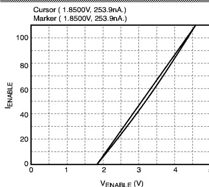
ENABLE Current vs. ENABLE Voltage
