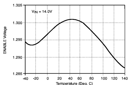
Enable Threshold Voltage vs. Temperature
