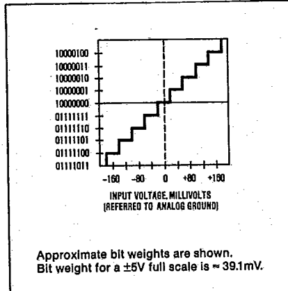
Figure 10. Bipolar Transfer Characteristic Around 0V
