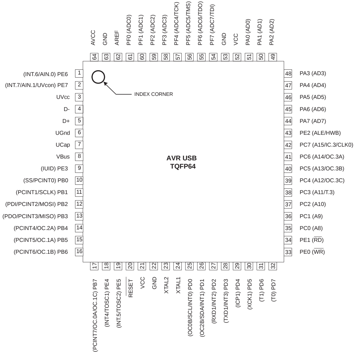
Figure 1-1. Pinout AT90USB64/128-TQFP
