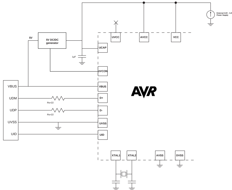
Figure 21-7. Host/OTG powered application with 3.0V to 3.4 I/O
