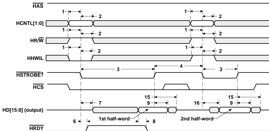
Figure 36. HPI16 Read Timing ( \overline{\text{HAS}} Not Used, Tied High)
