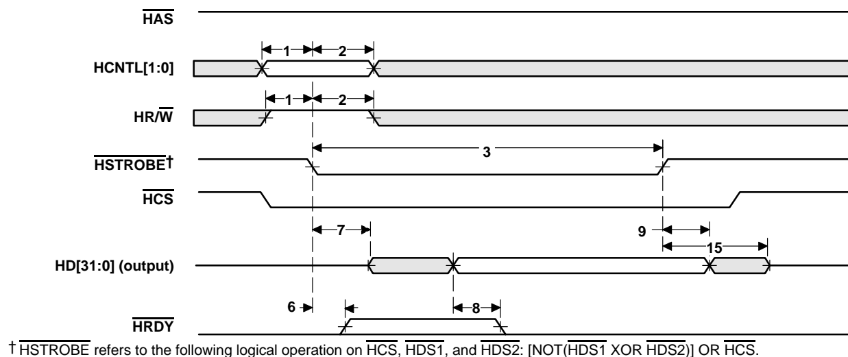
Figure 40. HPI32 Read Timing ( \overline{HAS} Not Used, Tied High)
