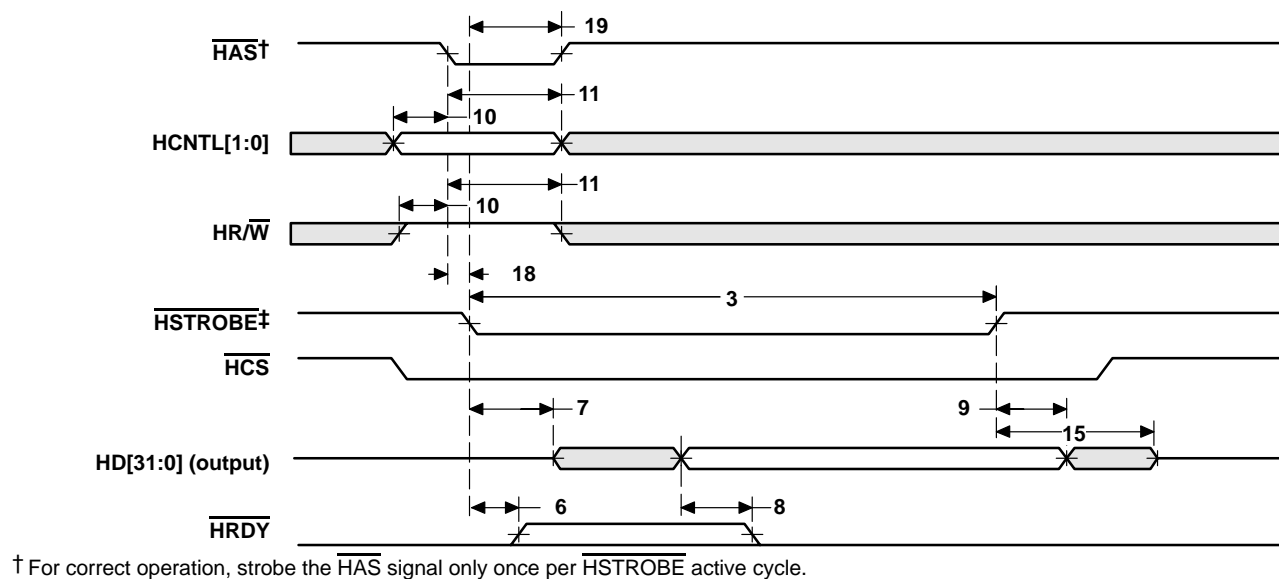
Figure 41. HPI32 Read Timing ( \overline{HAS} Used)
