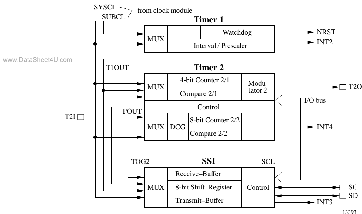
Figure 26. UTCM block diagram
