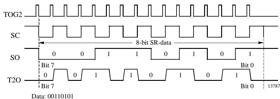
Figure 55. Manchester modulation 1
