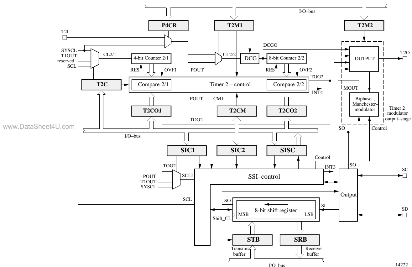
Figure 52. Combination Timer 2 and SSI
