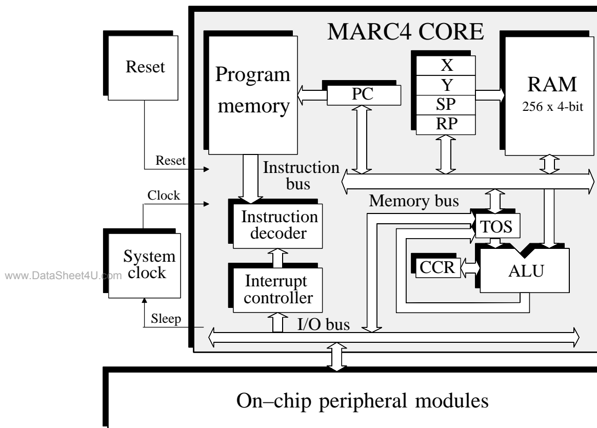
Figure 3. MARC4 core
