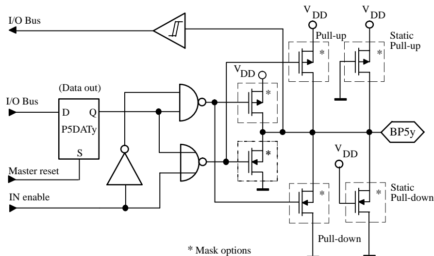
Figure 23. Bidirectional Port 5
