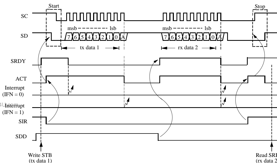
Figure 48. Example of I 2 C receive dialog
