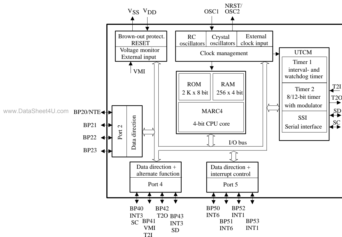
Figure 1. Block diagram of the T44C080-V
