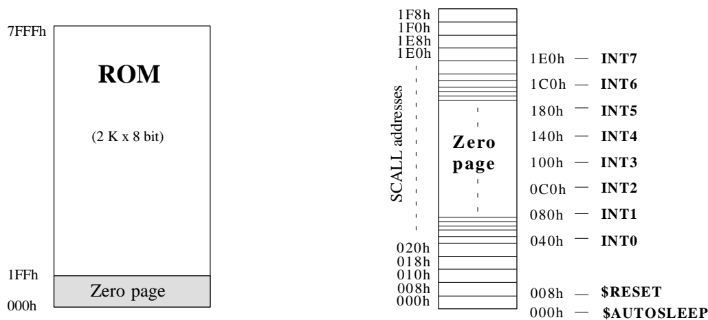
Figure 4. ROM map of T44C080-V
