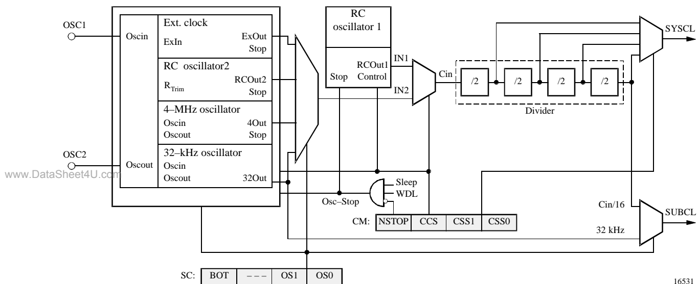
Figure 14. Clock module
