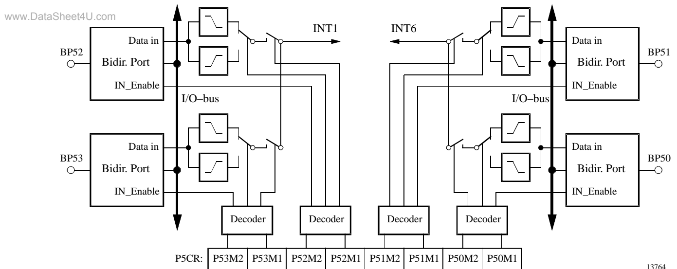
Figure 24. Port 5 external interrupts
