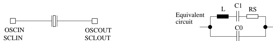
Figure 58. Crystal equivalent circuit
