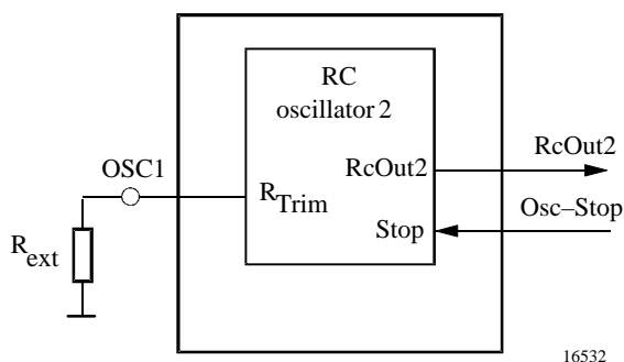
Figure 17. RC-oscillator 2
