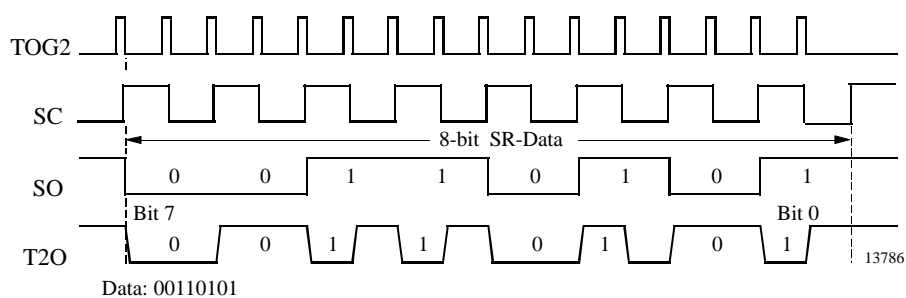
Figure 39. Biphase modulation
