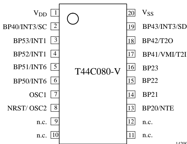
Figure 2. Pinning SSO20 package
