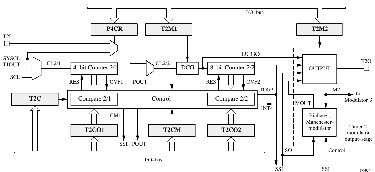
Figure 29. Timer 2
