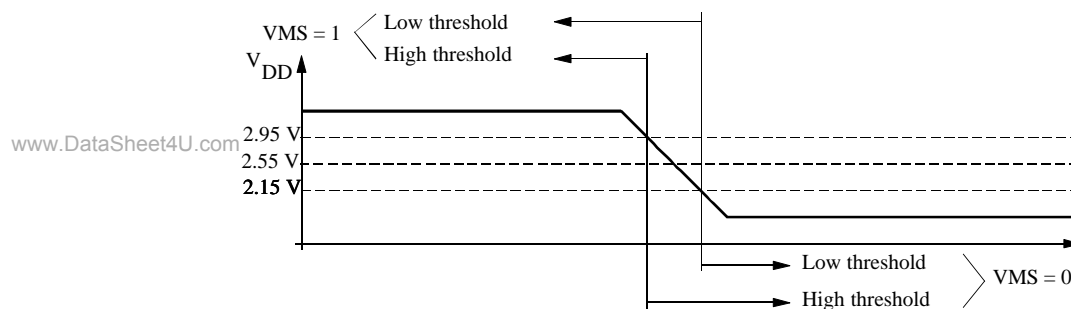
Figure 12. Internal supply voltage supervisor
