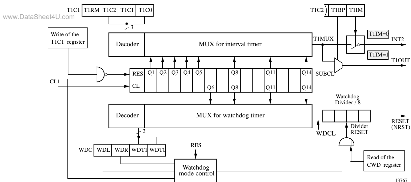
Figure 28. Timer 1 and watchdog
