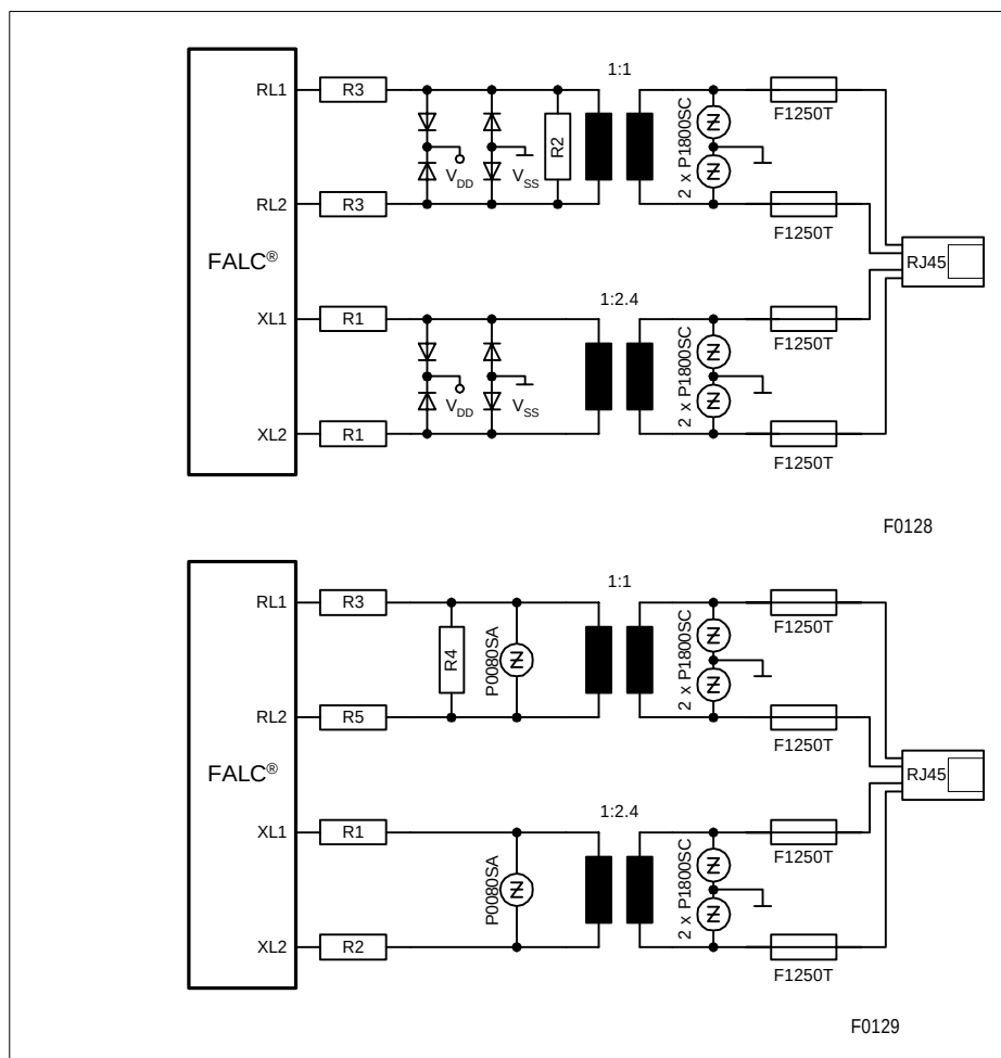
Figure 83 Protection Circuitry
