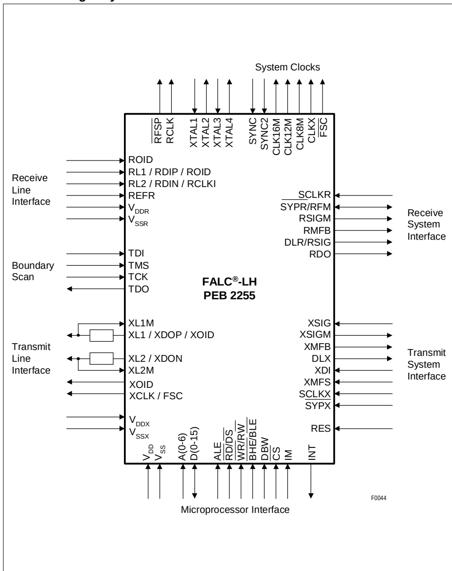
Figure 1 Logic Symbol
