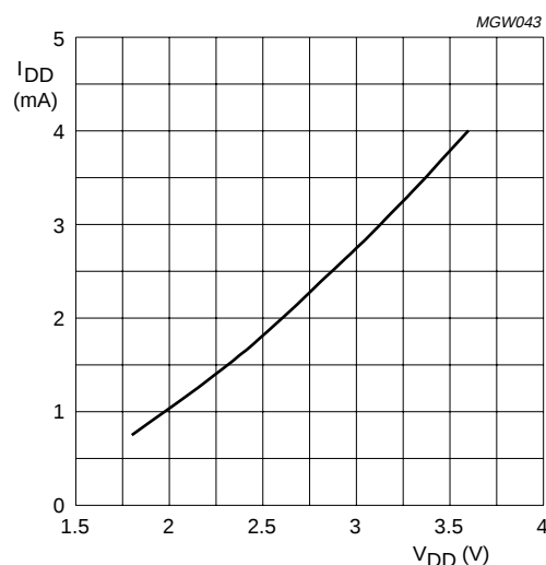
Fig.38 Typical operating current as a function of V_{DD} , T_{amb} = 25\text{ }^{\circ}\text{C} ; 100% CPU load (mean value over all instructions).
