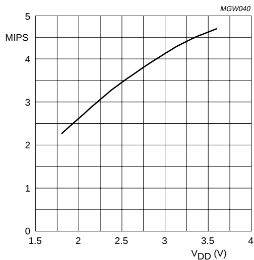
Fig.35 Typical CPU performance as a function of V_{DD} , T_{amb} = 25\text{ }^{\circ}\text{C} (mean value over all instructions).
