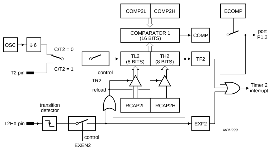
Fig.20 Timer 2 in Auto-reload mode (DCEN = 0).
