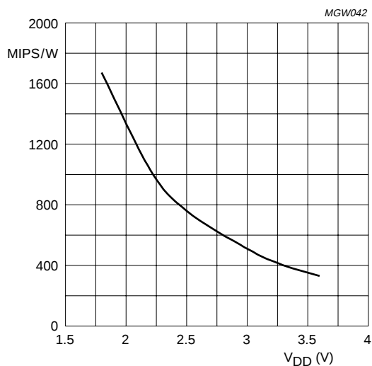
Fig.37 Typical CPU efficiency as a function of V_{DD} , T_{amb} = 25\text{ }^{\circ}\text{C} (mean value over all instructions).
