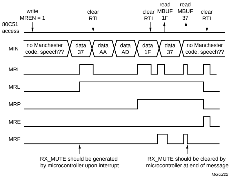
Fig.27 Data reception timing diagram.
