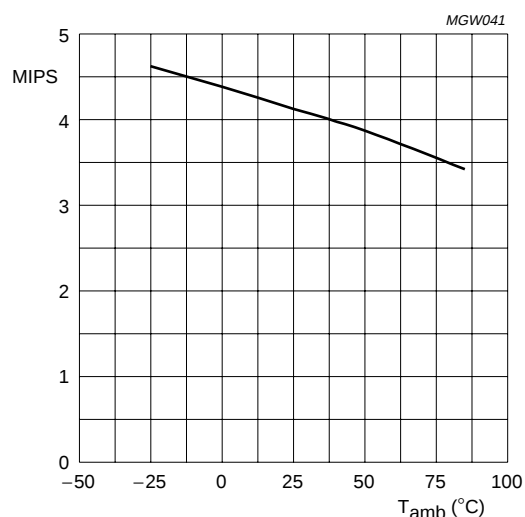
Fig.36 Typical CPU performance as a function of T_{amb} , V_{DD} = 3\text{ V} (mean value over all instructions).
