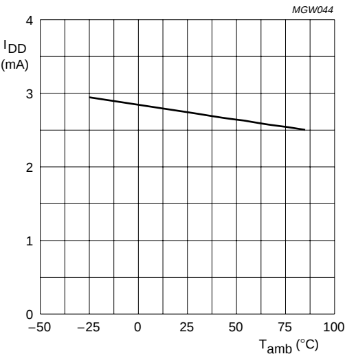
Fig.39 Typical operating current as a function of T_{amb} , V_{DD} = 3.0 V; 100% CPU load (mean value over all instructions).
