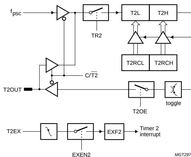
Fig.22 Timer 2 in Clock output mode.
