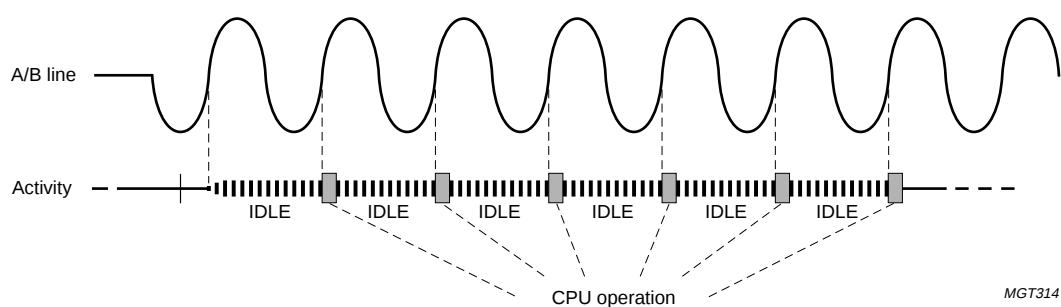
Fig.34 Ring-detection sequence.
