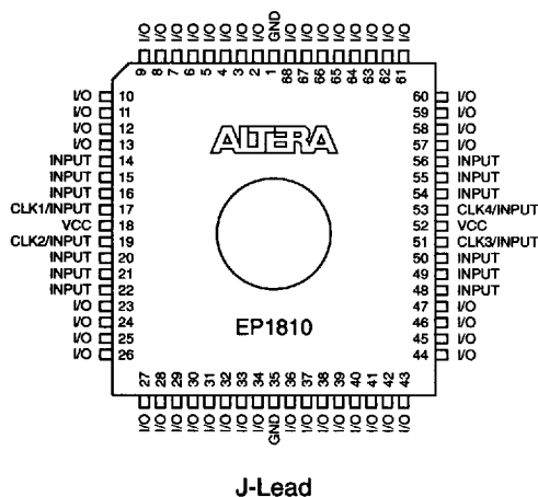
Figure 7. EP1810 Package Pin-Out Diagrams
