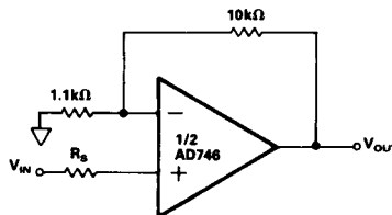
Figure 27. THD Measurement, Follower Circuit
