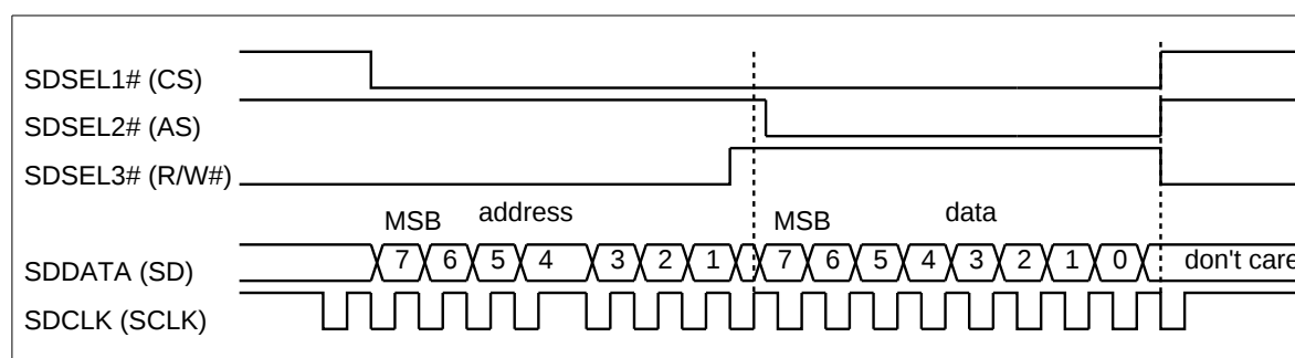
Figure 1. HSP3824 Serial Port Timing Diagram (Read Operation)
