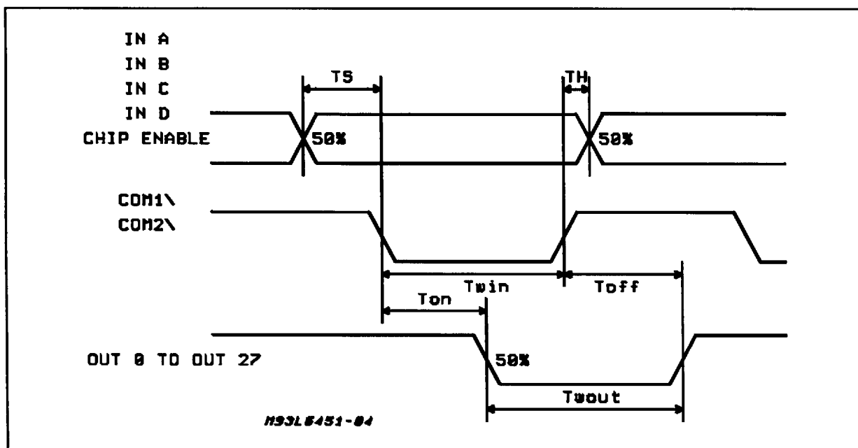
Figure 1: Timing Waveforms
