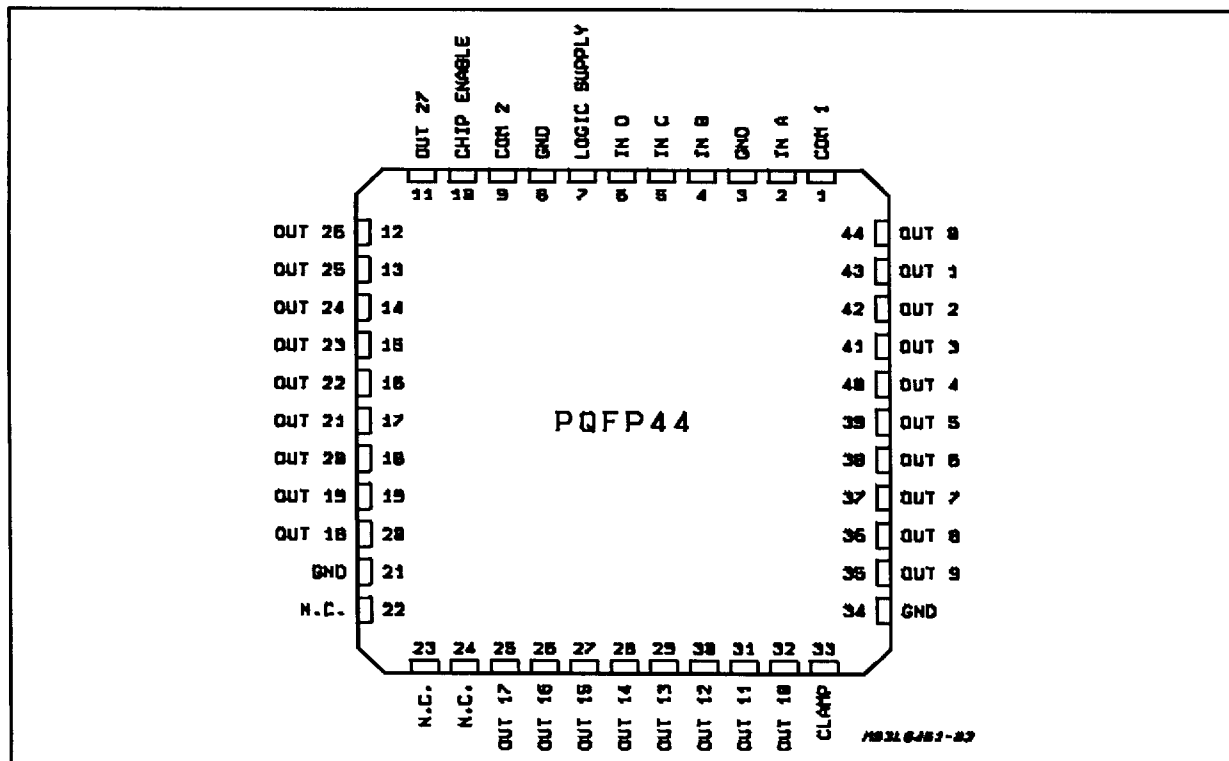
PQFP44 PIN CONNECTION (Top view)
