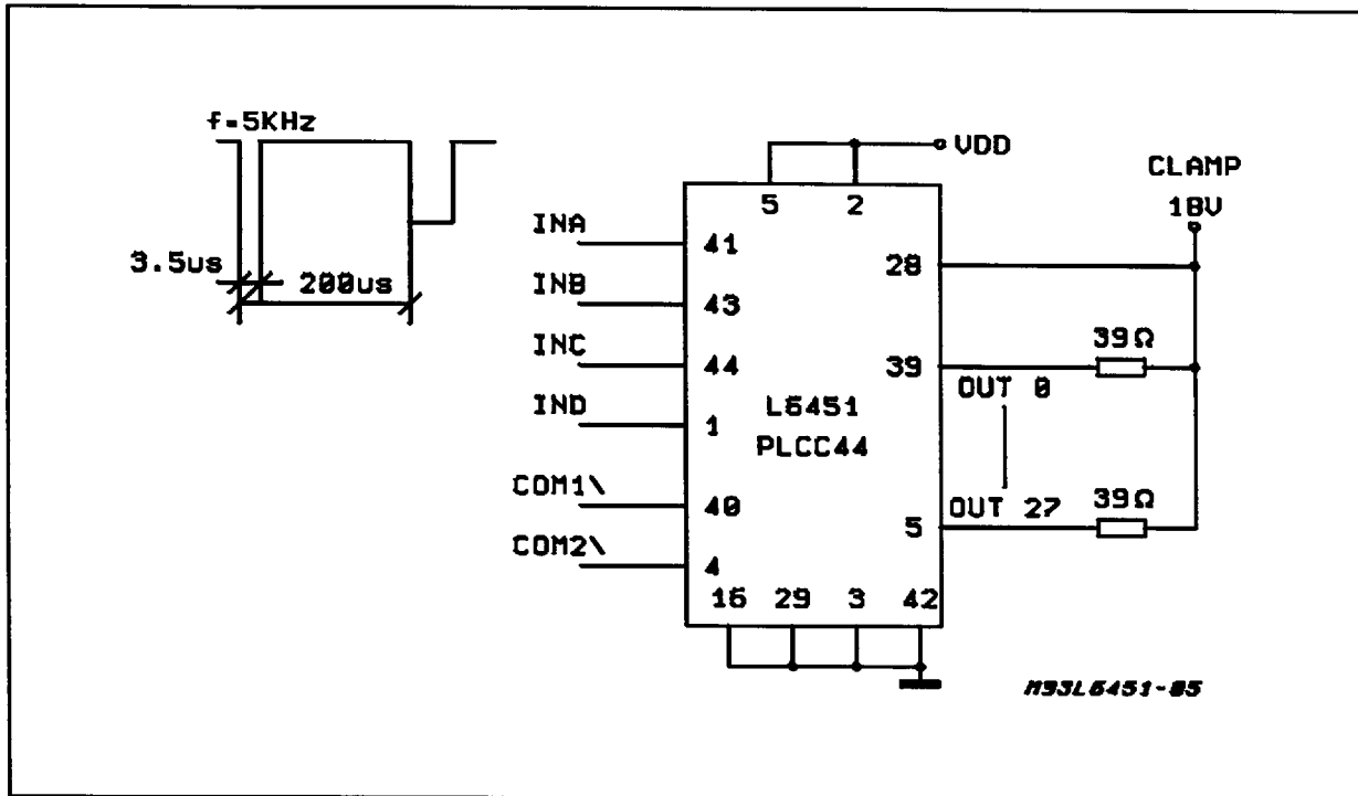
Figure 2: Application Circuit
