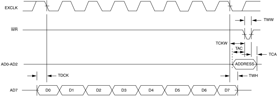
WRITE TIMING DIAGRAM (SERIAL VERSION)
