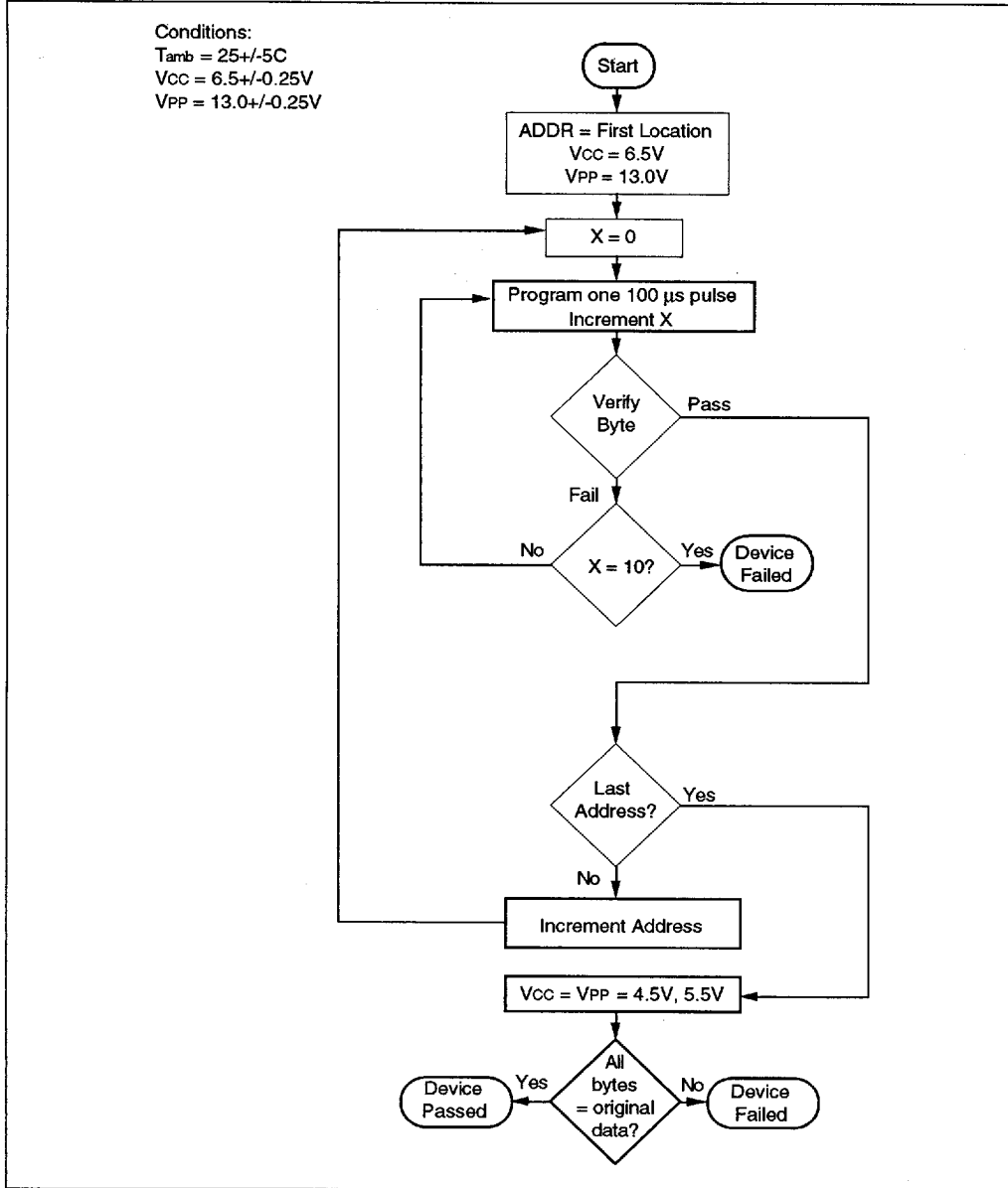
FIGURE 2-1: PROGRAMMING EXPRESS ALGORITHM
