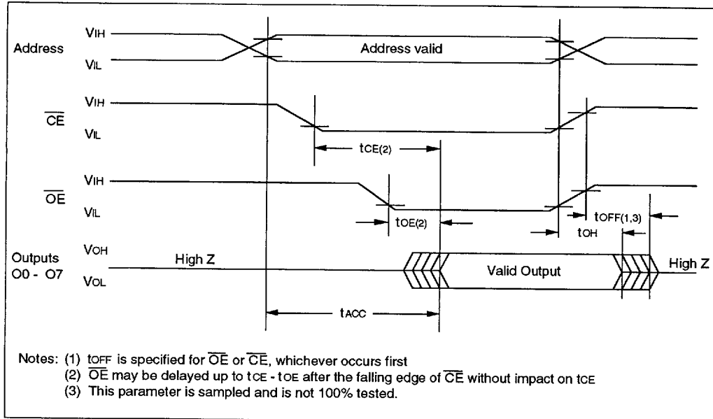
FIGURE 1-1: READ WAVEFORMS
