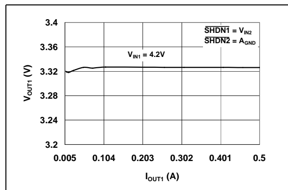
FIGURE 2-12: V_{OUT1} vs. I_{OUT1} ( V_{OUT1} = 3.3\text{V} ).
