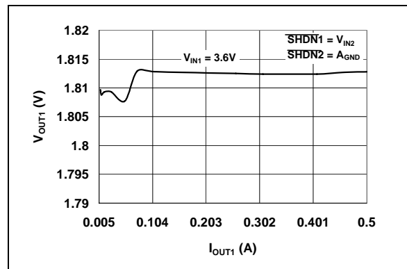
FIGURE 2-11: V_{OUT1} vs. I_{OUT1} ( V_{OUT1} = 1.8\text{V} ).
