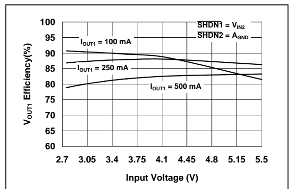
FIGURE 2-6: V_{OUT1} Output Efficiency vs. Input Voltage ( V_{OUT1} = 1.8\text{V} ).
