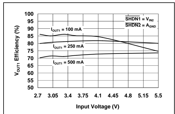
FIGURE 2-4: V_{OUT1} Output Efficiency vs. Input Voltage ( V_{OUT1} = 1.2\text{V} ).
