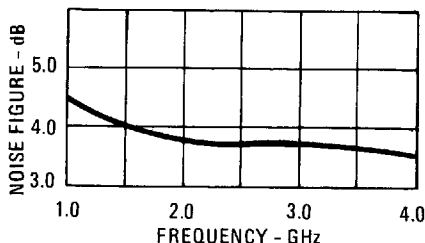
Noise Figure
