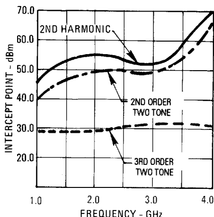
Intercept Point
