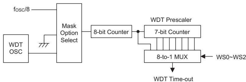
Watchdog Timer
