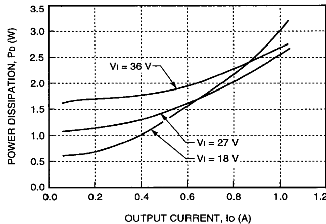
Figure 17. 12 V Output Power Dissipation vs. Output Current
