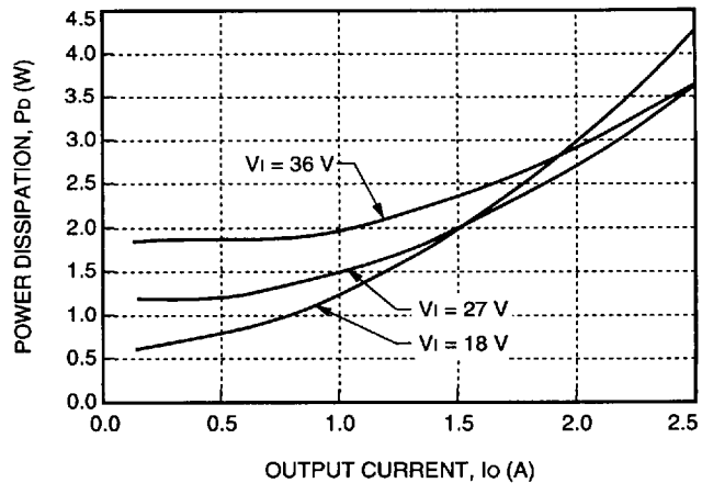
Figure 16. 5 V Output Power Dissipation vs. Output Current
