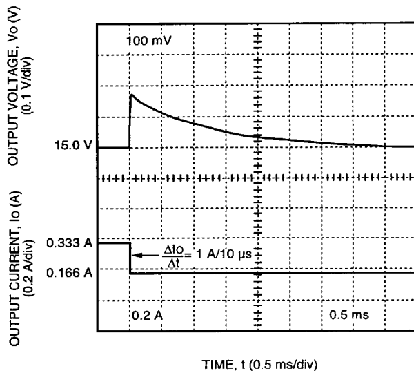
Figure 6. CC025 Dual-Output-Series Typical 15 V Output Voltage Response to a Step Load Change from 50% to 25% of I_{o,max} at V_i = V_{i,nom} and T_c = 25^\circ C
