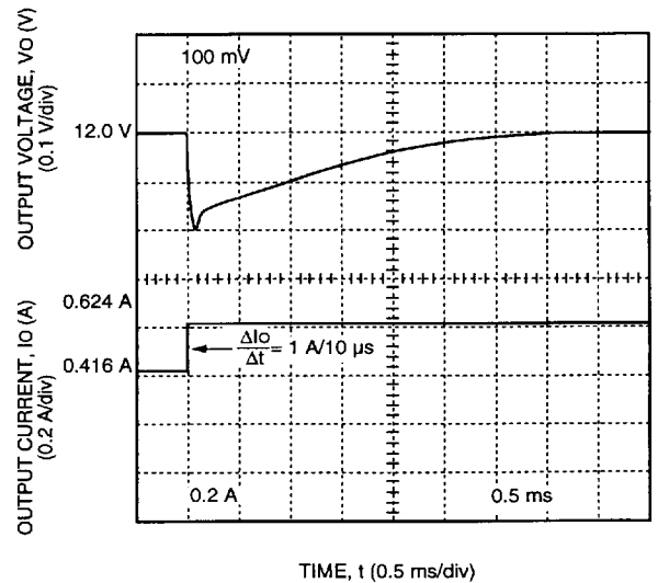
Figure 8. CC025 Dual-Output-Series Typical 12 V Output Voltage Response to a Step Load Change from 50% to 75% of I_{o,max} at V_i = V_{i,nom} and T_c = 25^\circ C
