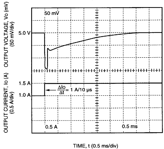
Figure 7. CC025 Dual-Output-Series Typical 5 V Output Voltage Response to a Step Load Change from 50% to 75% of I_{o,max} at V_i = V_{i,nom} and T_c = 25^\circ C
