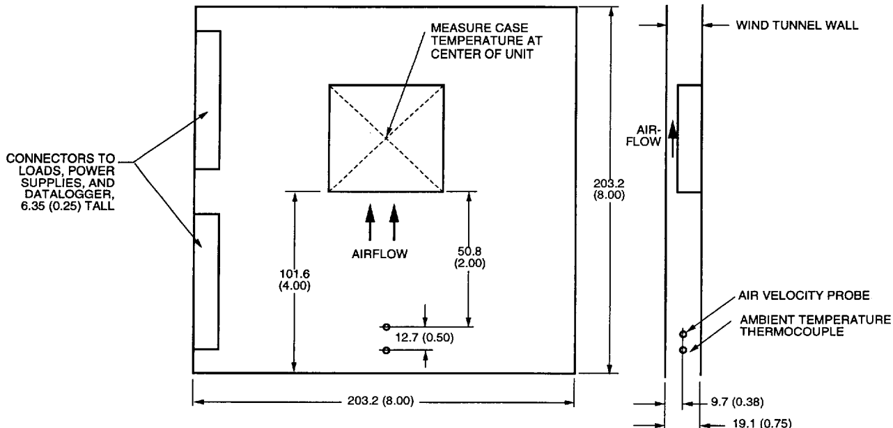
Figure 15. Thermal Test Setup
