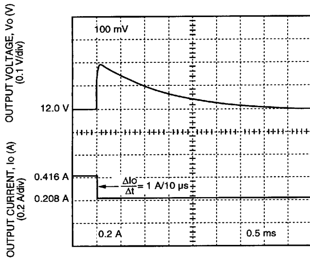
Figure 5. CC025 Dual-Output-Series Typical 12 V Output Voltage Response to a Step Load Change from 50% to 25% of I_{o,max} at V_i = V_{i,nom} and T_c = 25^\circ C
