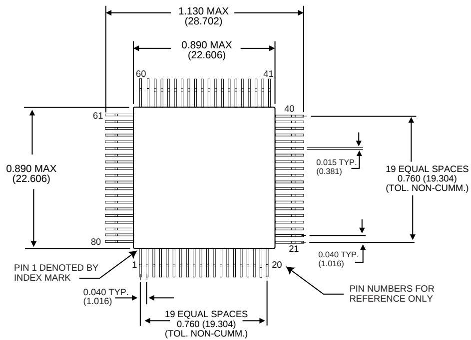
TOP VIEW
