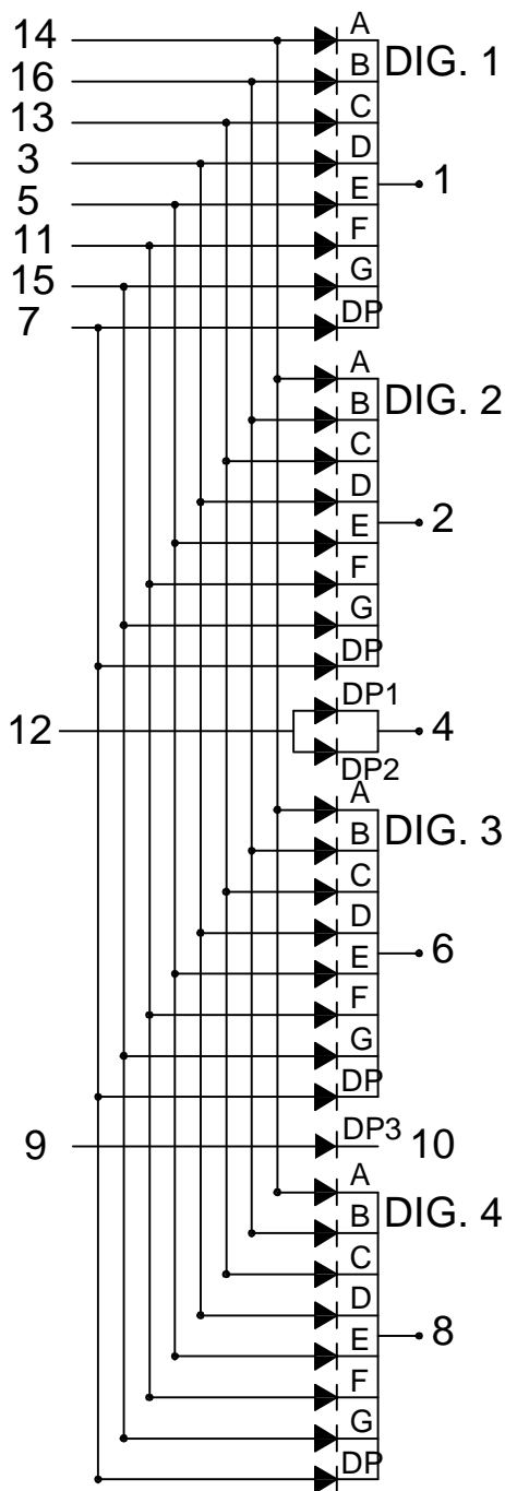
LFD4155-XX/RP33-PF
