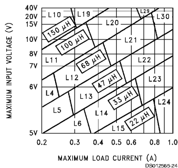
FIGURE 4. LM2595-3.3
