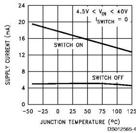
Operating Quiescent Current
