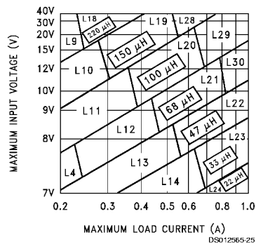
FIGURE 5. LM2595-5.0
