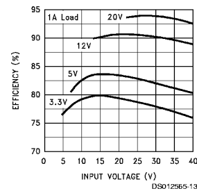
Efficiency
