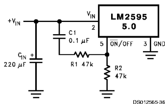
FIGURE 21. Delayed Startup
