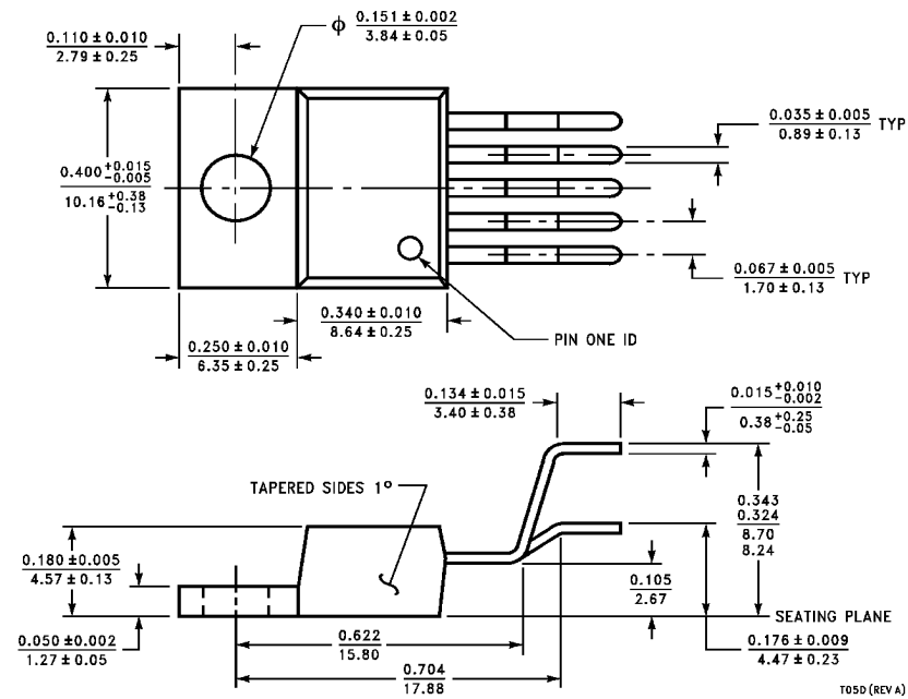
5-Lead TO-220 (T) Order Number LM2595T-3.3, LM2595T-5.0, LM2595T-12 or LM2595T-ADJ NS Package Number T05D
