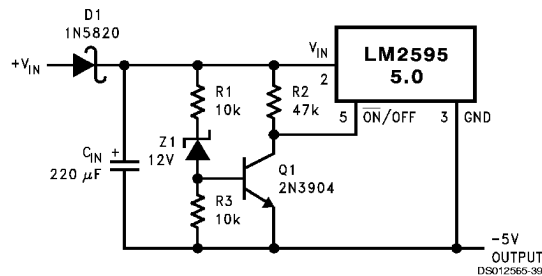
FIGURE 24. Undervoltage Lockout with Hysteresis for Inverting Regulator
