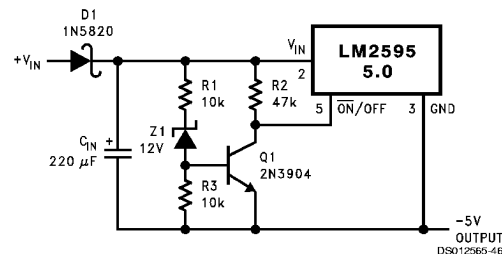
FIGURE 23. Undervoltage Lockout for Inverting Regulator
