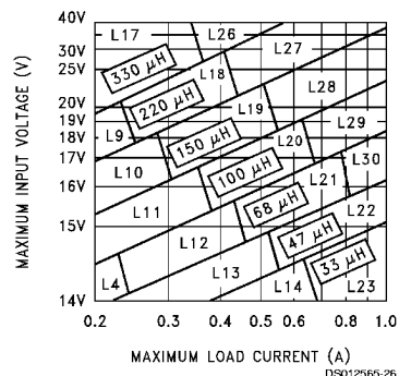
FIGURE 6. LM2595-12
