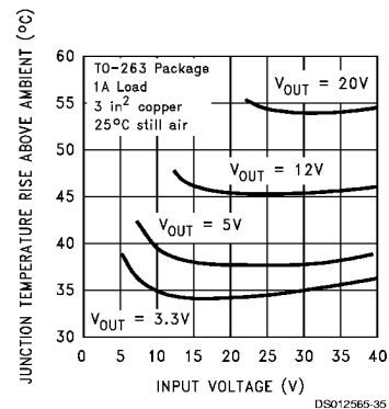
FIGURE 19. Junction Temperature Rise, TO-220
