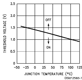
ON/OFF Threshold Voltage
