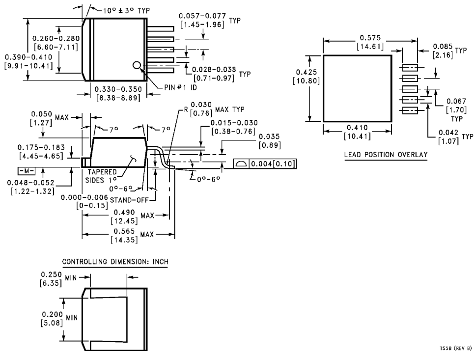
5-Lead TO-263 Surface Mount Package (S) Order Number LM2595S-3.3, LM2595S-5.0, LM2595S-12 or LM2595S-ADJ NS Package Number TS5B
