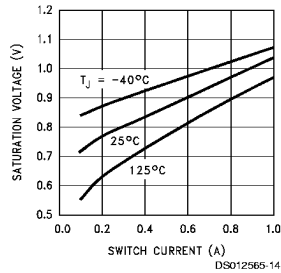
Switch Saturation Voltage
