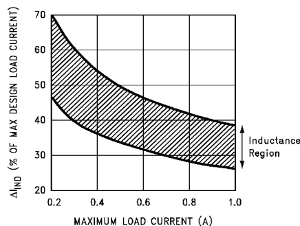
FIGURE 16. ( \Delta I_{LND} ) Peak-to-Peak Inductor Ripple Current (as a Percentage of the Load Current) vs Load Current
