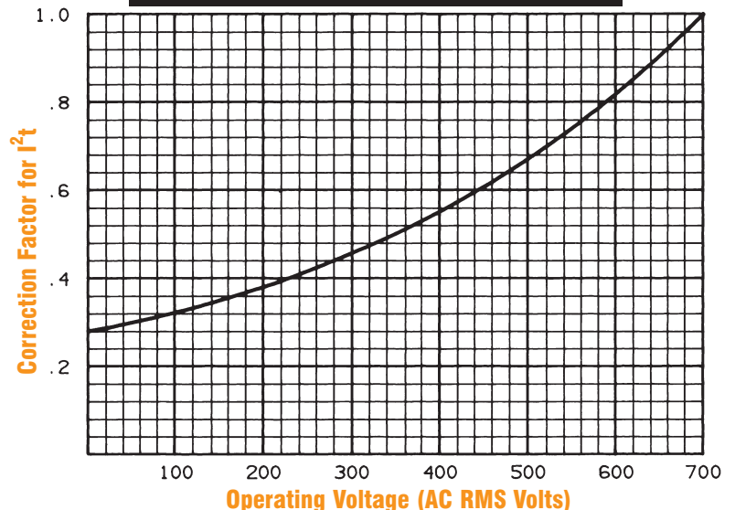
Clearing I 2 t vs. AC Operating Voltage
