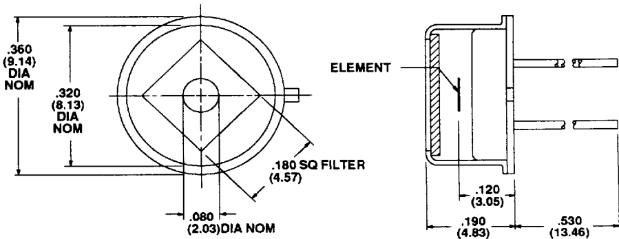
DIMENSIONS IN INCHES (mm) PIN CIRCLE .200 (5.08); LEAD DIA .017 (0.432)
