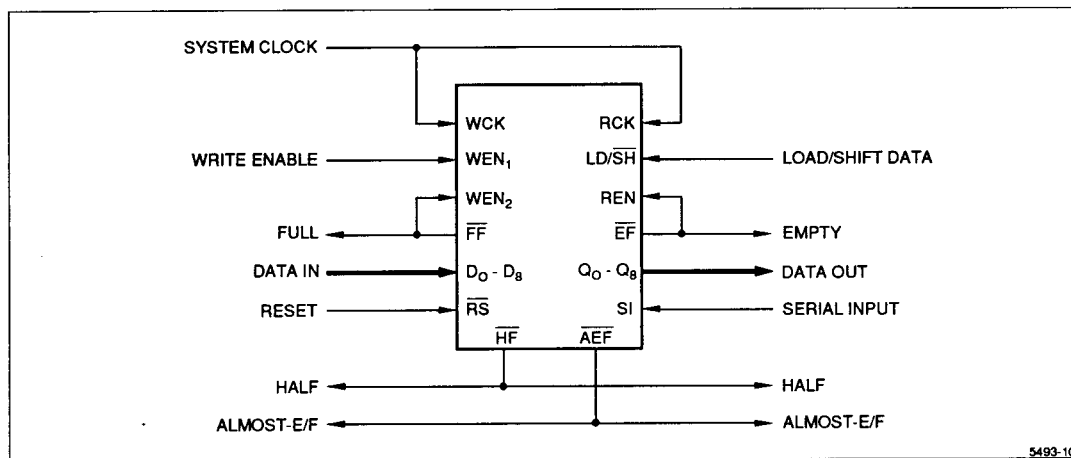
Figure 11. Synchronous Operation
