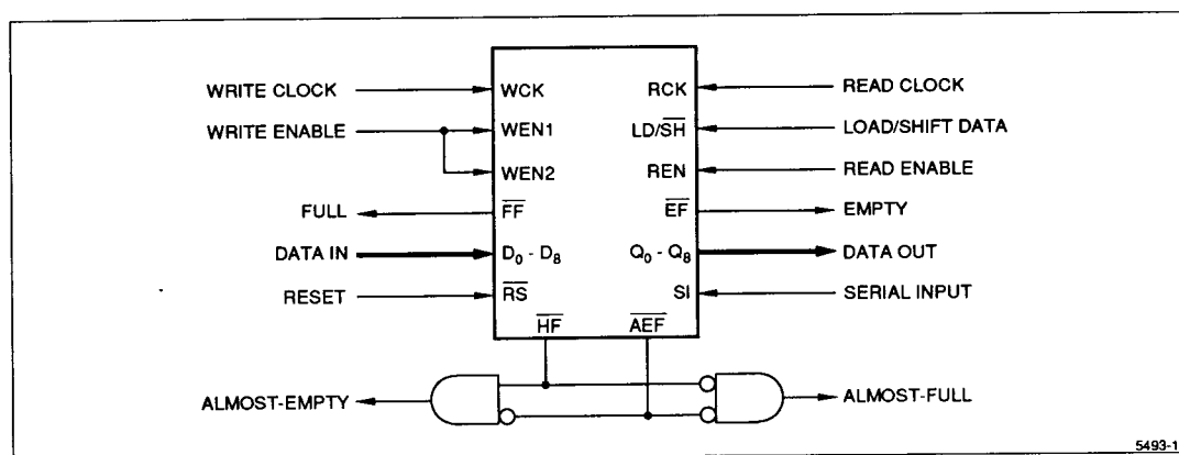
Figure 12. Asynchronous Operation
