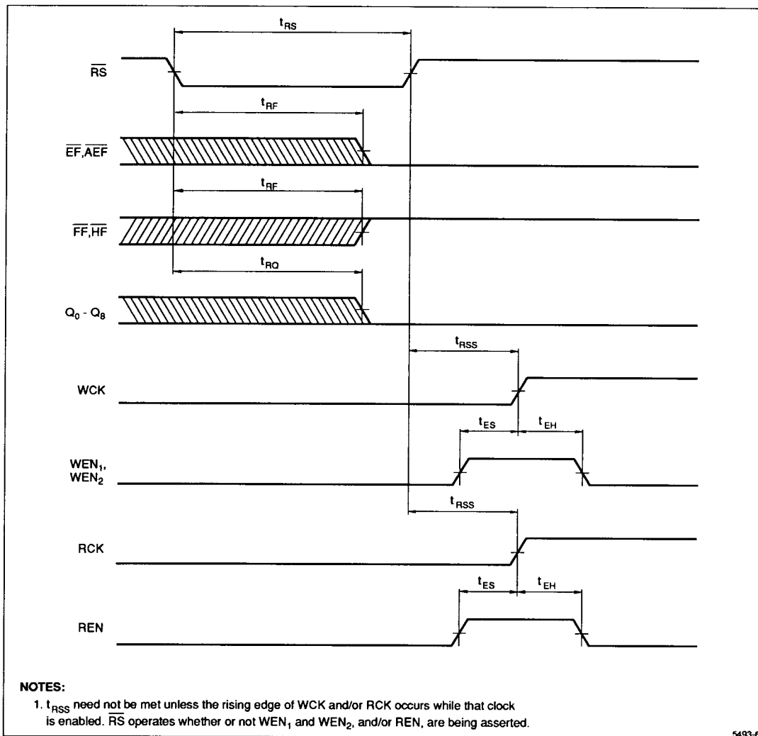
Figure 7. Reset Timing
