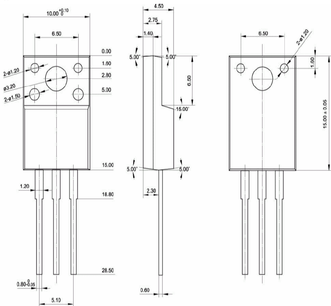
Fig.2 Outline dimensions
