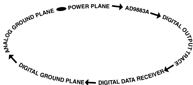
Figure 13. Current Loop
