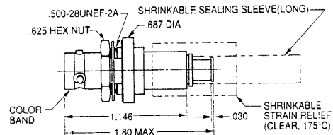
BULKHEAD CABLE JACK TOOL CRIMP 3-lug BJ79C-△ 2-lug BJ79CTL-△ 4-lug BJ79CFL-△ Threaded BJ379C-△
