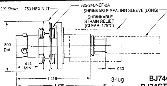
INSULATED BULKHEAD CABLE JACK TOOL CRIMP
