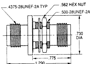
FEED-THRU BULKHEAD JACK Threaded
