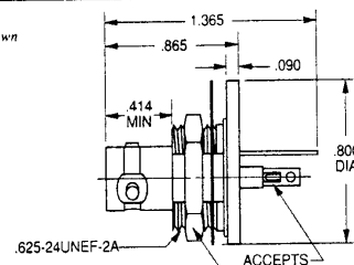
INSULATED BULKHEAD JACK REAR MOUNT, SOLDER POT
