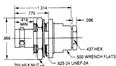
3-lug BJ74-△ 2-lug BJ74TL-△ 4-lug BJ74FL-△ Threaded BJ374-△
