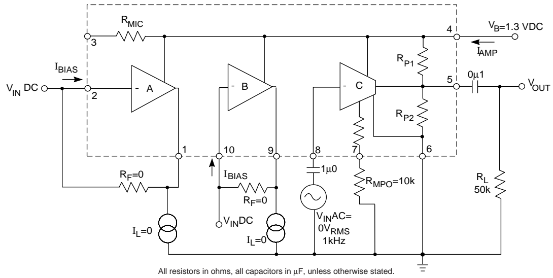
Fig. 1 Test Circuit
