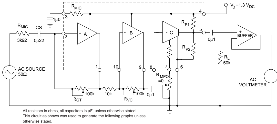
Fig. 5 Characterization Circuit
