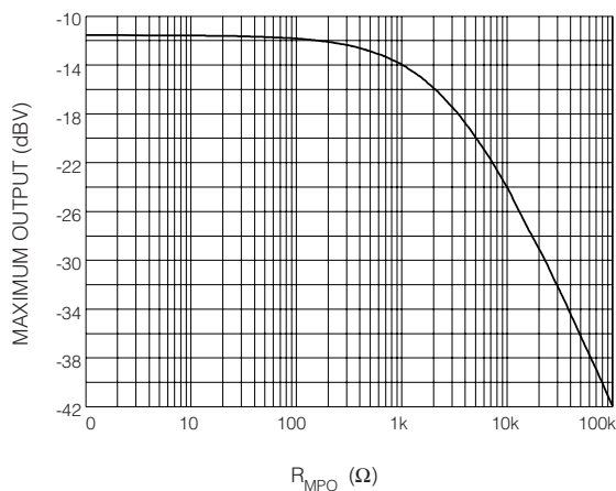
Fig. 12 Maximum Output vs R_{MPO} (as in Fig. 1, V_{INAC} = -15\text{dBV} )
