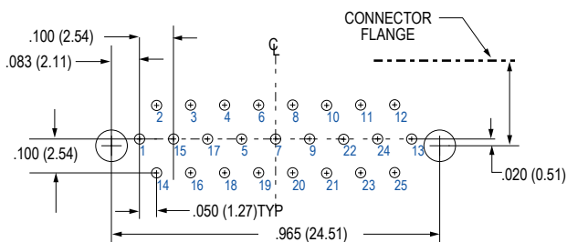
25 Contacts
