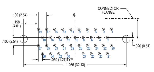
37 Contacts
