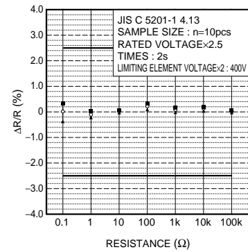
Fig.7 過負荷
