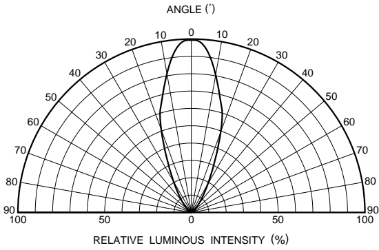
Fig.2 SLI-560 Directional pattern
