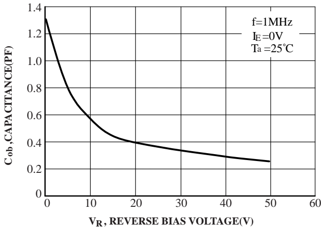
FIG.35 Output Capacitance
