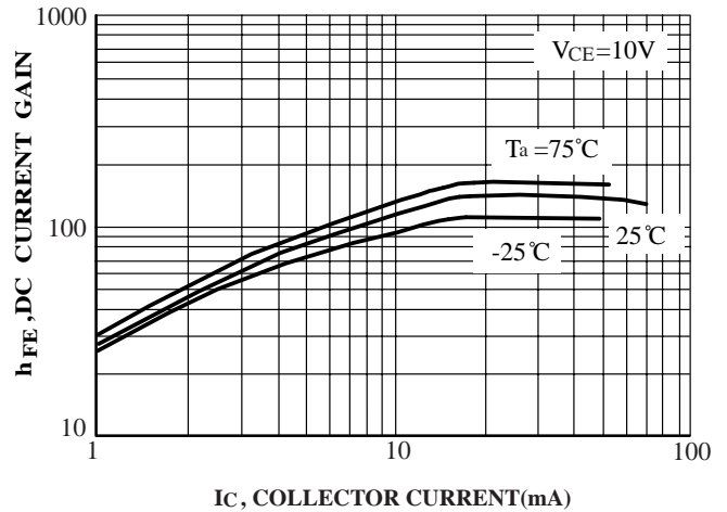
IC, COLLECTOR CURRENT(mA) FIG.9 DC Current Gain
